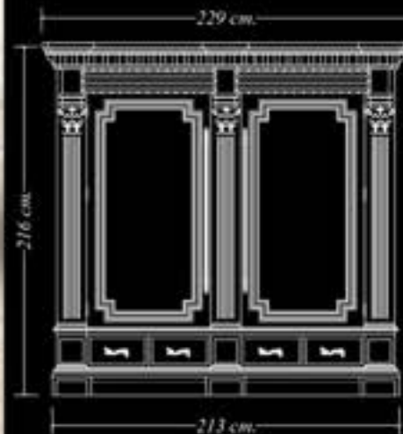
455C Dsc Buffet Front View
